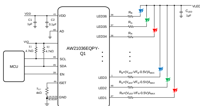
Figure 1 AW21036EQPY-Q1 Application Circuit
