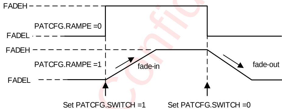
Figure 15 Manual Control Mode
