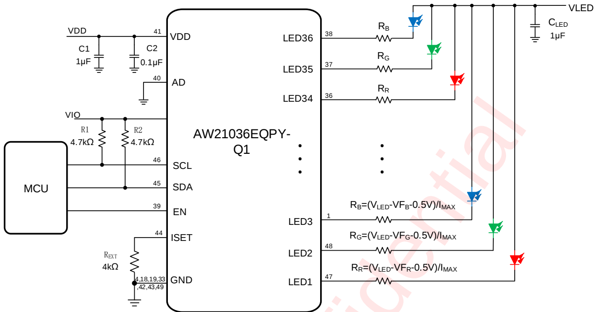
Figure 4 AW21036EQPY-Q1 Application Circuit
