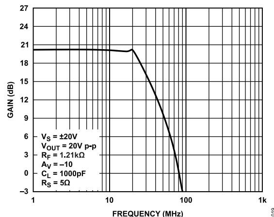
Figure 19. Large Signal Frequency Response, A_V = -10 , V_S = \pm 20 V, V_{OUT} = 20 V p-p, R_F = 1.21 k \Omega , C_L = 1000 pF, R_S = 5 \Omega
