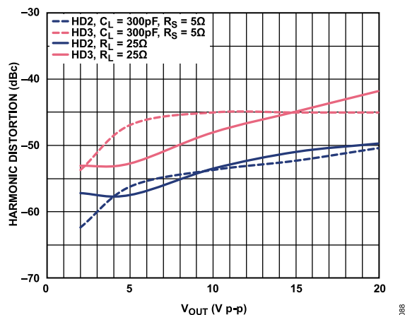
Figure 48. Harmonic Distortion vs. V_{OUT} , V_S = \pm 20 V, Frequency = 10 MHz, R_F = 1.21 k \Omega , A_V = -10
