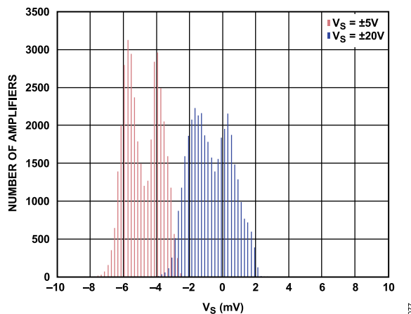
Figure 67. Input Offset Voltage Distribution, V_S = \pm 5\text{ V} , V_S = \pm 20\text{ V}
