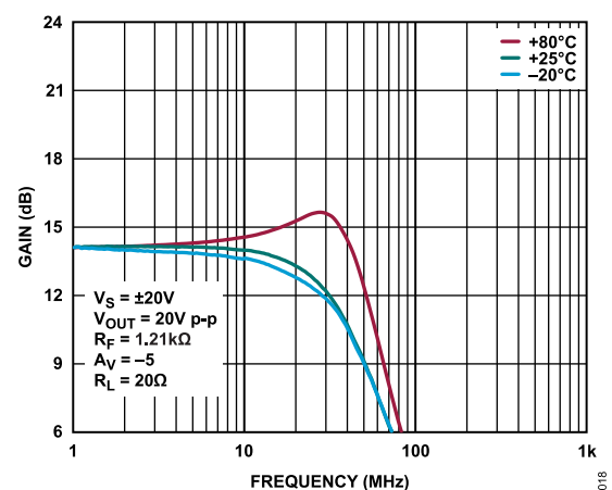
Figure 18. Large Signal Frequency Response vs. Case Temperature, A_V = -5 , V_S = \pm 20 V, V_{OUT} = 20 V p-p, R_F = 1.21 k \Omega , R_L = 20 \Omega
