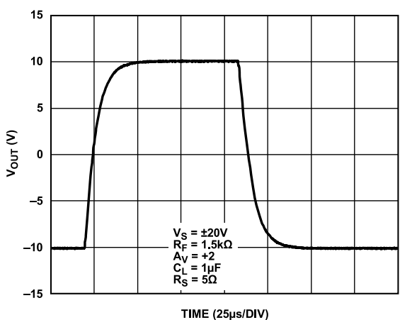
Figure 39. Large Signal Pulse Response, A_V = +2 , V_S = \pm 20 V, V_{OUT} = 20 V p-p, R_F = 1.5 k \Omega , C_L = 1 \mu F, R_S = 5 \Omega
