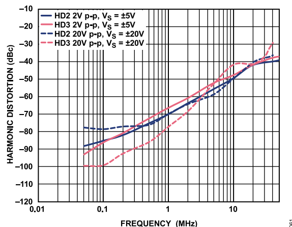
Figure 49. Harmonic Distortion vs. Frequency, R_L = 25 \Omega , R_F = 1.21 k \Omega , A_V = -10
