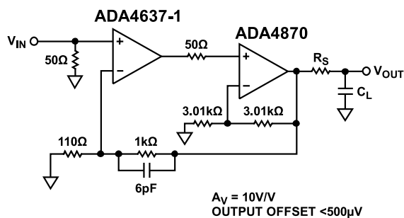
Figure 77. Composite Amplifier
