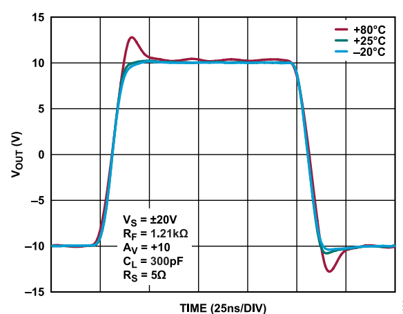
Figure 33. Large Signal Pulse Response vs. Case Temperature, A_V = +10 , V_S = \pm 20 V, V_{OUT} = 20 V p-p, R_F = 1.21 k \Omega , C_L = 300 pF, R_S = 5 \Omega
