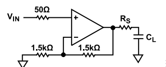
Figure 69. Circuit for Capacitive Load Drive
