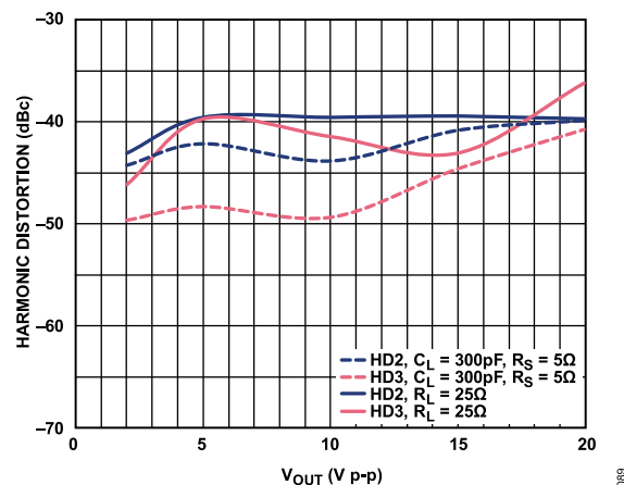
Figure 51. Harmonic Distortion vs. V_{OUT} , V_S = \pm 20 V, Frequency = 30 MHz, R_F = 1.21 k \Omega , A_V = -10
