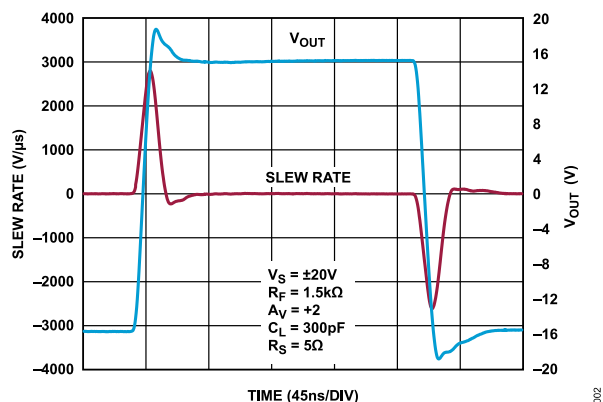
Figure 52. Large Signal Instantaneous Slew Rate, A_V = +2 , V_S = \pm 20 V, R_F = 1.5 k \Omega , C_L = 300 pF, R_S = 5 \Omega
