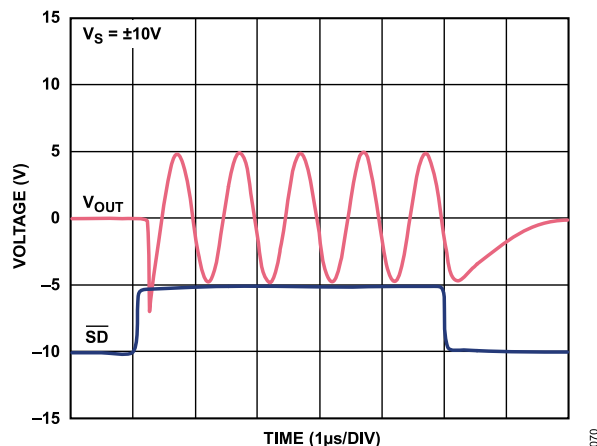
Figure 60. Turn-On/Turn-Off Time, V_S = \pm 10\text{ V}
