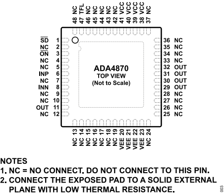
Figure 3. Pin Configuration
