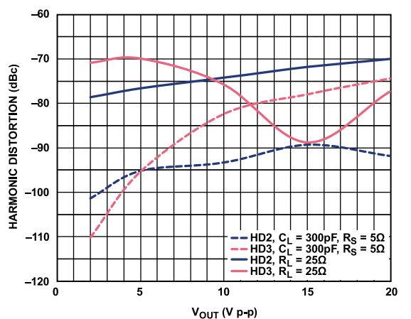
Figure 50. Harmonic Distortion vs. V_{OUT} , V_S = \pm 20 V, Frequency = 1 MHz, R_F = 1.21 k \Omega , A_V = -10
