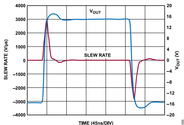
Figure 55. Large Signal Instantaneous Slew Rate, A_V = +2 , V_S = \pm 20 V, R_F = 1.5 k \Omega , R_L = 25 \Omega
