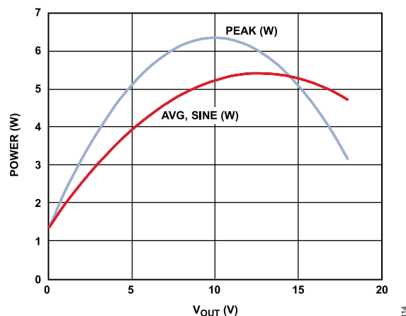
Figure 73. Average Sine and Peak Power vs. V_{OUT} , V_S = \pm 20\text{ V} , R_L = 20\Omega
