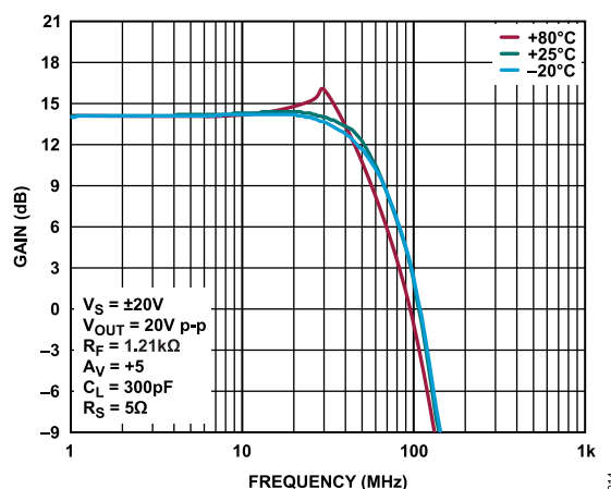
Figure 14. Large Signal Frequency Response vs. Case Temperature, A_V = +5 , V_S = \pm 20V , V_{OUT} = 20V p-p, R_F = 1.21k\Omega , C_L = 300pF , R_S = 5\Omega
