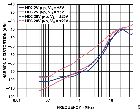
Figure 46. Harmonic Distortion vs. Frequency, C_L = 300 pF, R_S = 5 \Omega , R_F = 1.21 k \Omega , A_V = -10
