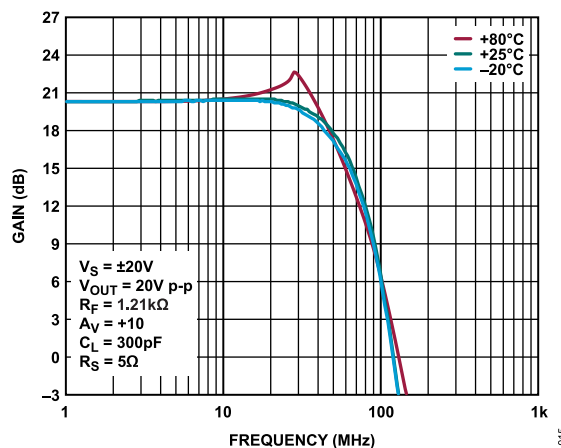
Figure 15. Large Signal Frequency Response vs. Case Temperature, A_V = +10 , V_S = \pm 20V , V_{OUT} = 20V p-p, R_F = 1.21k\Omega , C_L = 300pF , R_S = 5\Omega
