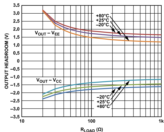
Figure 56. Output Headroom vs. R_{LOAD} Over Case Temperature, V_S = \pm 20 V
