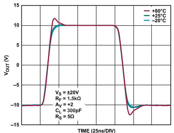
Figure 31. Large Signal Pulse Response vs. Case Temperature, A_V = +2 , V_S = \pm 20 V, V_{OUT} = 20 V p-p, R_F = 1.5 k \Omega , C_L = 300 pF, R_S = 5 \Omega
