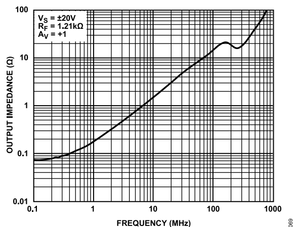
Figure 54. Enabled Closed-Loop Output Impedance vs. Frequency
