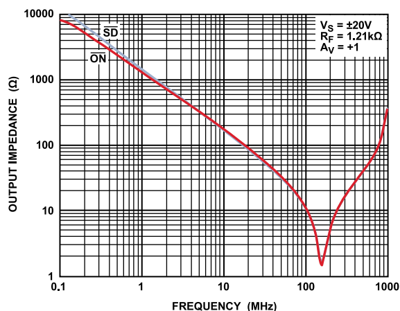
Figure 57. Disabled Closed-Loop Output Impedance vs. Frequency
