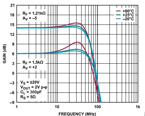
Figure 21. Small Signal Frequency Response vs. Case Temperature, V_S = \pm 20 V, V_{OUT} = 2 V p-p, C_L = 300 pF, R_S = 5 \Omega
