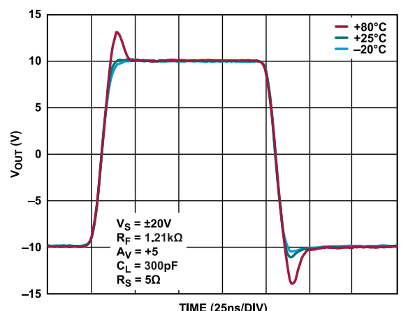
Figure 32. Large Signal Pulse Response vs. Case Temperature, A_V = +5 , V_S = \pm 20 V, V_{OUT} = 20 V p-p, R_F = 1.21 k \Omega , C_L = 300 pF, R_S = 5 \Omega
