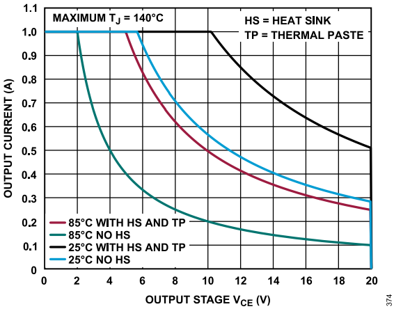
Figure 74. Safe Operating Area for Evaluation Board from Figure 75 at 25°C and 85°C Ambient Temperature With and Without Heat Sink, No Air Flow
