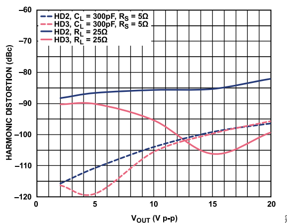
Figure 47. Harmonic Distortion vs. V_{OUT} , V_S = \pm 20 V, Frequency = 100 kHz, R_F = 1.21 k \Omega , A_V = -10
