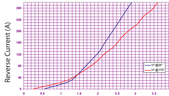
Reverse Voltage Drop (V) Figure 10b
