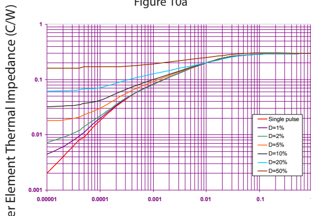
Pulse Duration (S) Figure 10c
