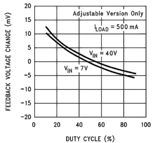
Feedback Voltage vs Duty Cycle
