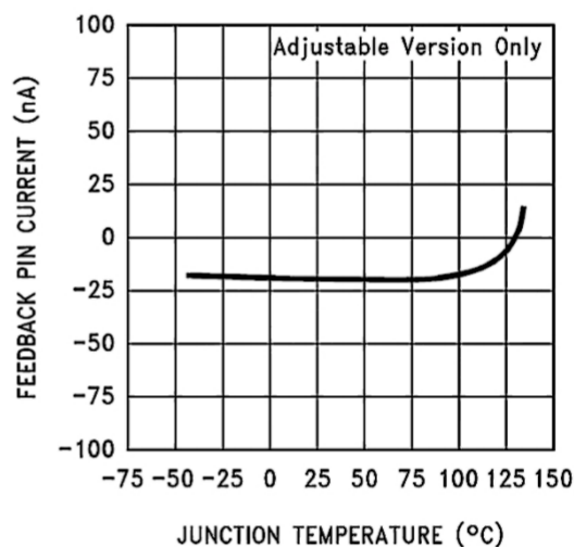
Feedback Pin Current
