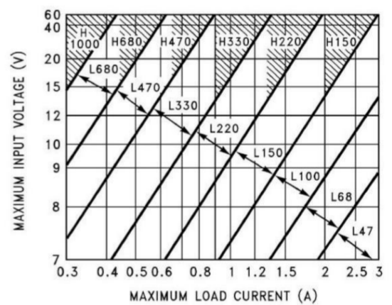
LM2576HV-5.0
