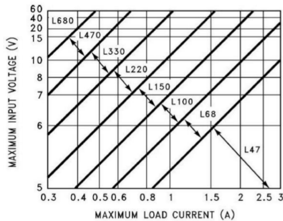
LM2576HV-3.3
