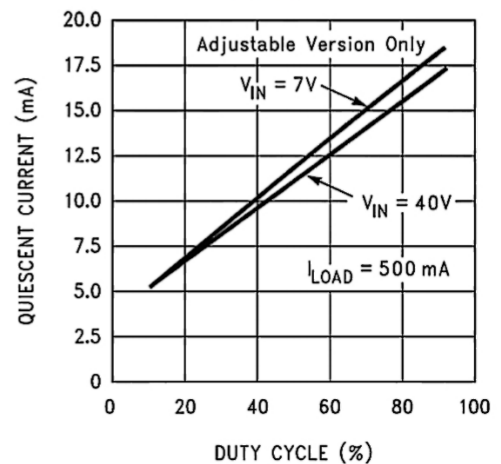
Quiescent Current vs Duty Cycle
