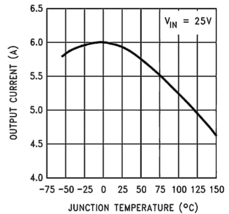
Current Limit
