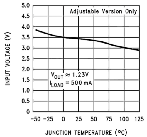
Minimum Operating Voltage
