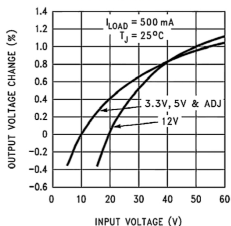
Line Regulation
