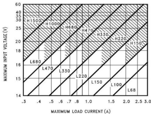
LM2576HV-12
