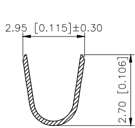
SECTION:A-A SCALE:1:1
