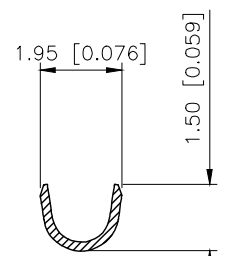
SECTION:B-B SCALE:1:1
