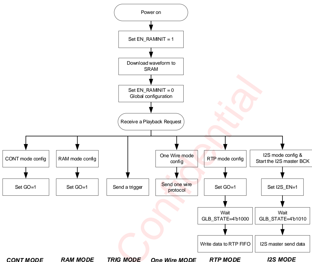
Figure 16 Power up and playback sequence
