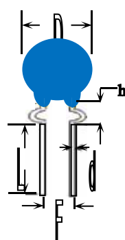
TYPE E: 平肩 Flat shoulder
