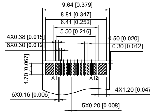
RECOMMENDED PCB LAYOUT(TOP VIEW) THICKNESS 0.80±0.05MM;DEFAULT TOLERANCE:±0.05
