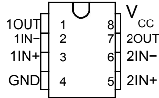
D, DGK, P, PS, PW and JG Package 8-Pin SOIC, VSSOP, PDIP, SO, TSSOP and CDIP (Top View)
