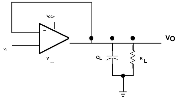
Figure 11. Unity-Gain Amplifier
