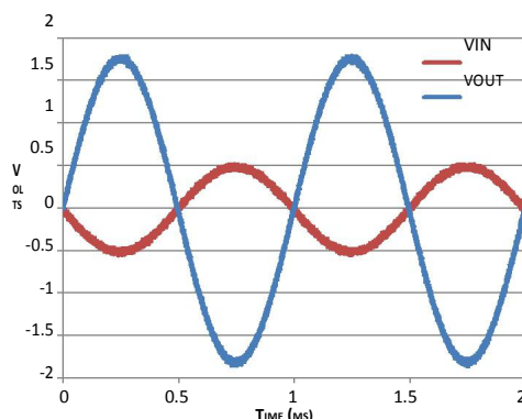
Figure 14. Input and Output Voltages of the Inverting Amplifier
