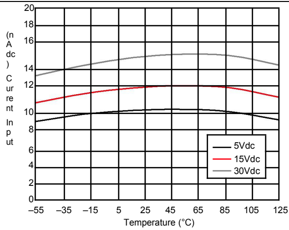
Figure 1. Input Current vs. Temperature
