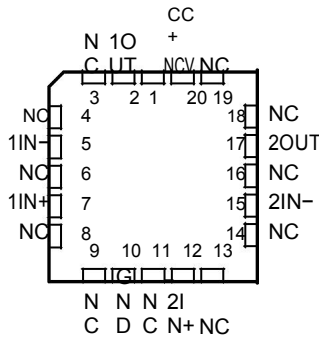
FK Package 20-Pin LCCC (Top View)
