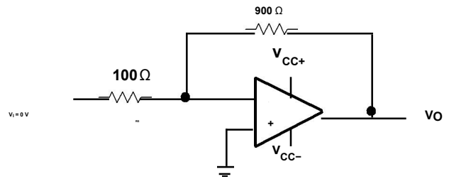
Figure 12. Noise-Test Circuit
