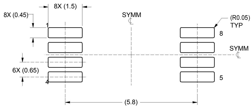
LAND PATTERN EXAMPLE SCALE:10X
