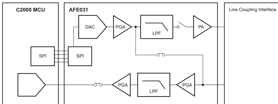
Figure 46. Rx Calibration Mode Configuration
