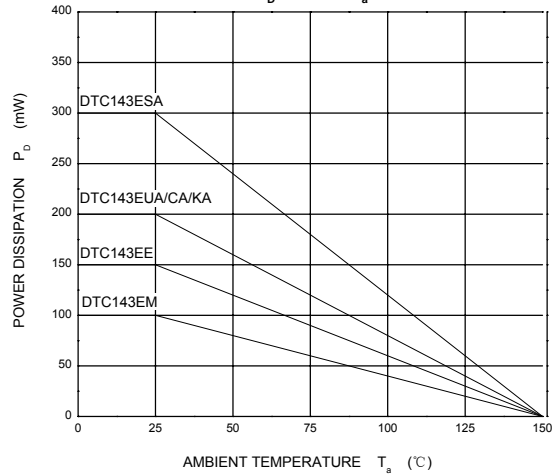
P_D - T_a
