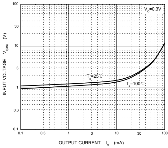
ON Characteristics
