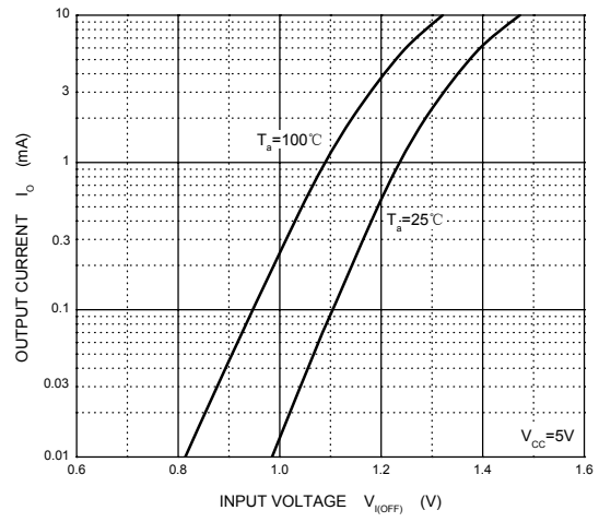
OFF Characteristics
