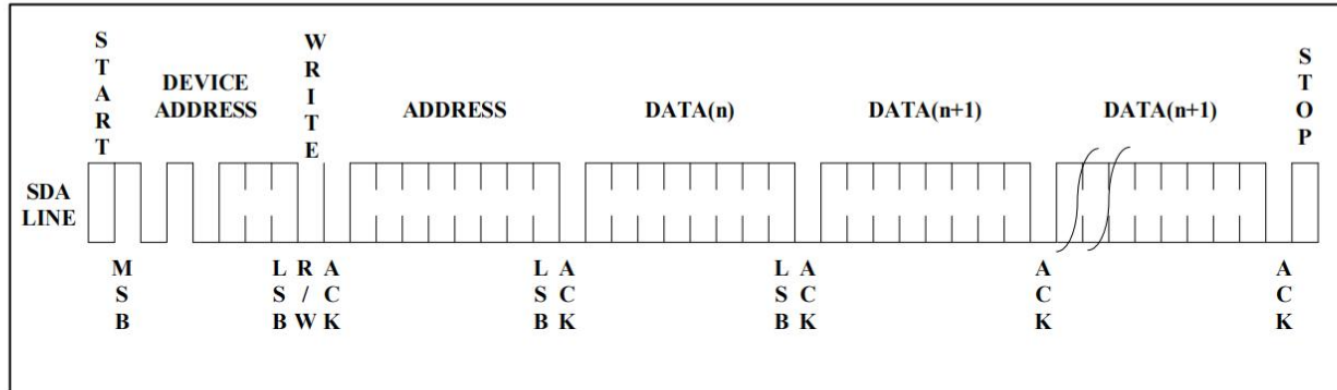
Figure 8. Page Write
