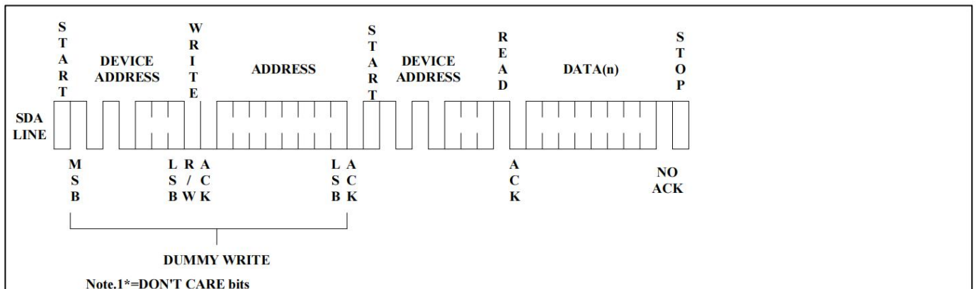
Figure 10. Random Read
