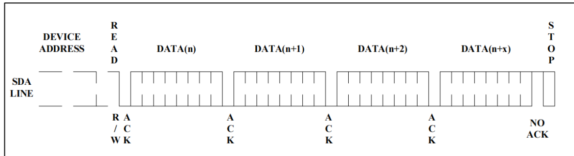
Figure 11. Sequential Read
