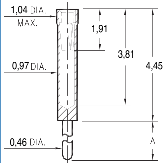
0461-X-15-XX-X1-XX-04-0 Solder mount in 0,51 min. mounting hole
