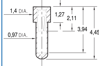
6214-0-15-XX-21-XX-10-0 Solder mount in 1,02 min mounting hole
