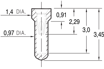
6023-0-15-XX-21-XX-10-0 Solder mount in 1,02 min mounting hole
