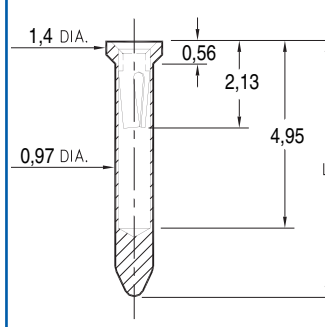
8579-0-15-XX-X1-XX-10-0 Solder mount in 1,02 min mounting hole
