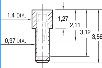
0569-0-15-XX-X1-XX-10-0 Solder mount in 1,02 min mounting hole
