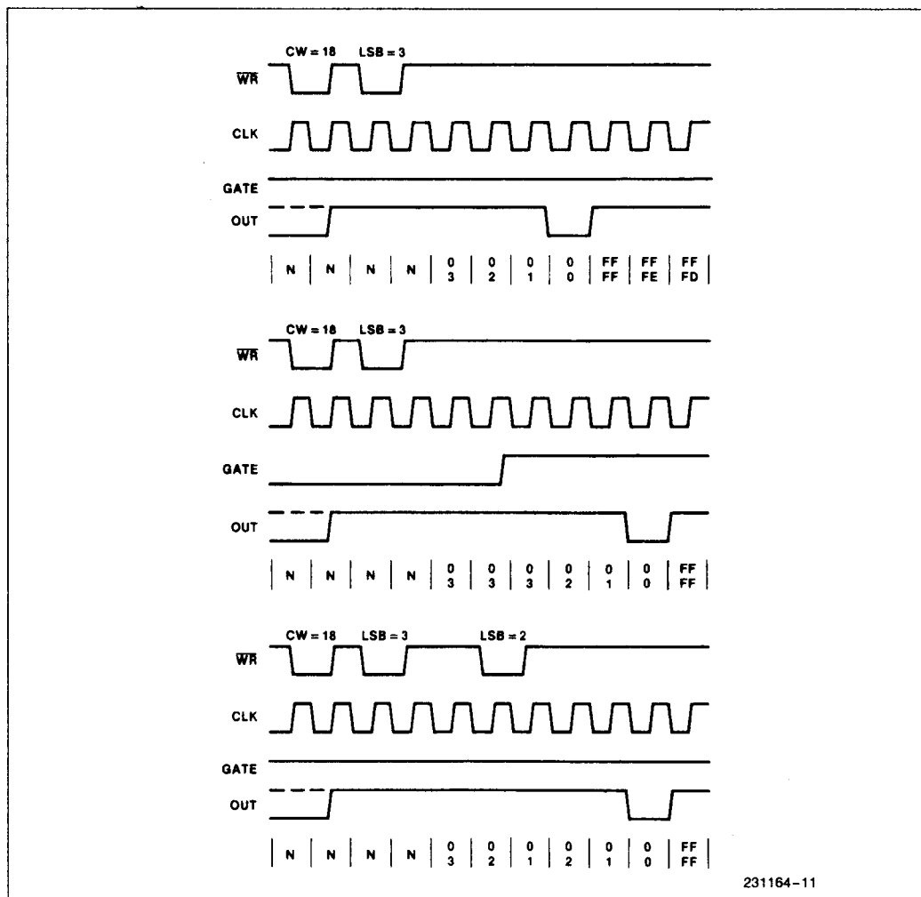
Figure 19. Mode 4
