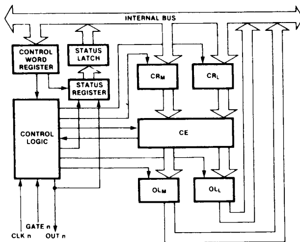
Figure 5. Internal Block Diagram of a Counter
