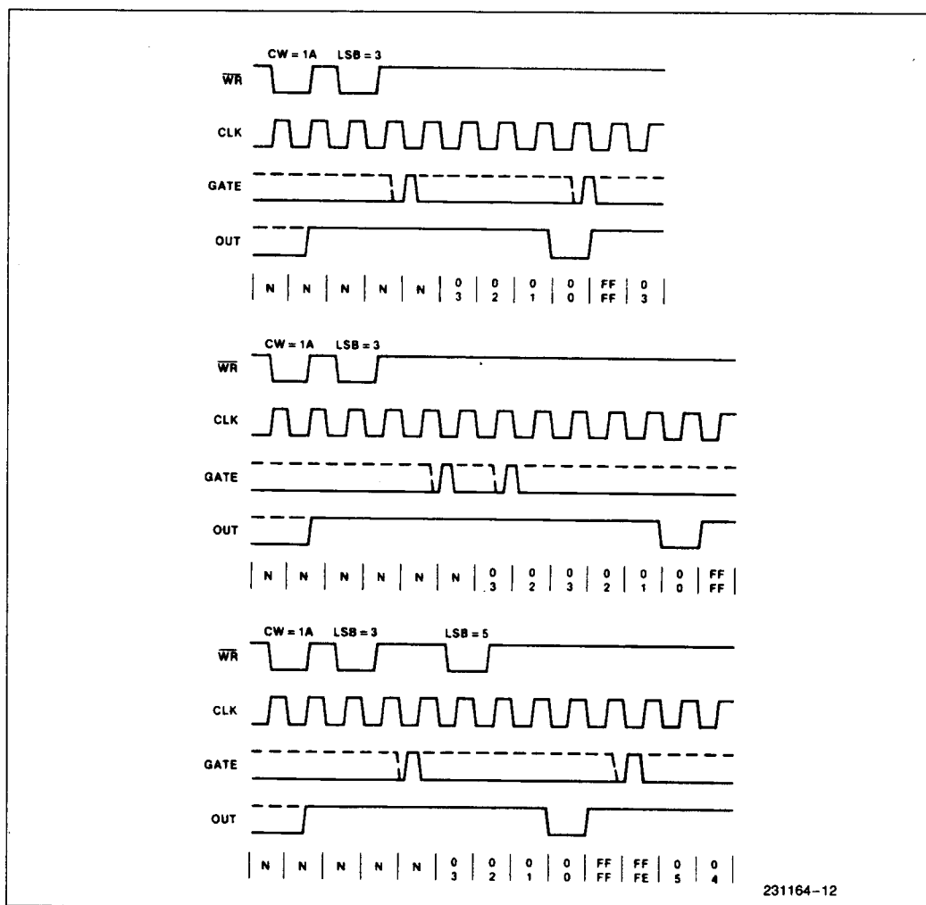
Figure 20. Mode 5
