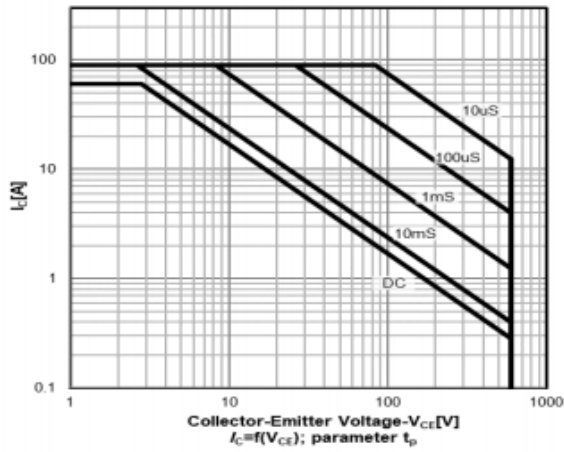
Safe operating area Ta=25 °C Non-Full PAK
