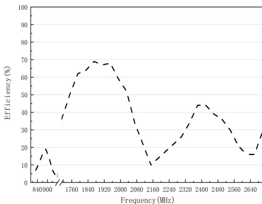
Figure 8. Total Efficiency
