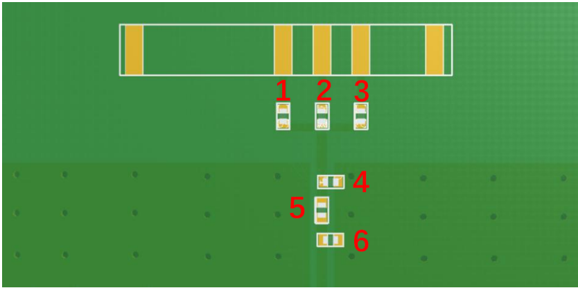
Figure 5. Matching Circuit
