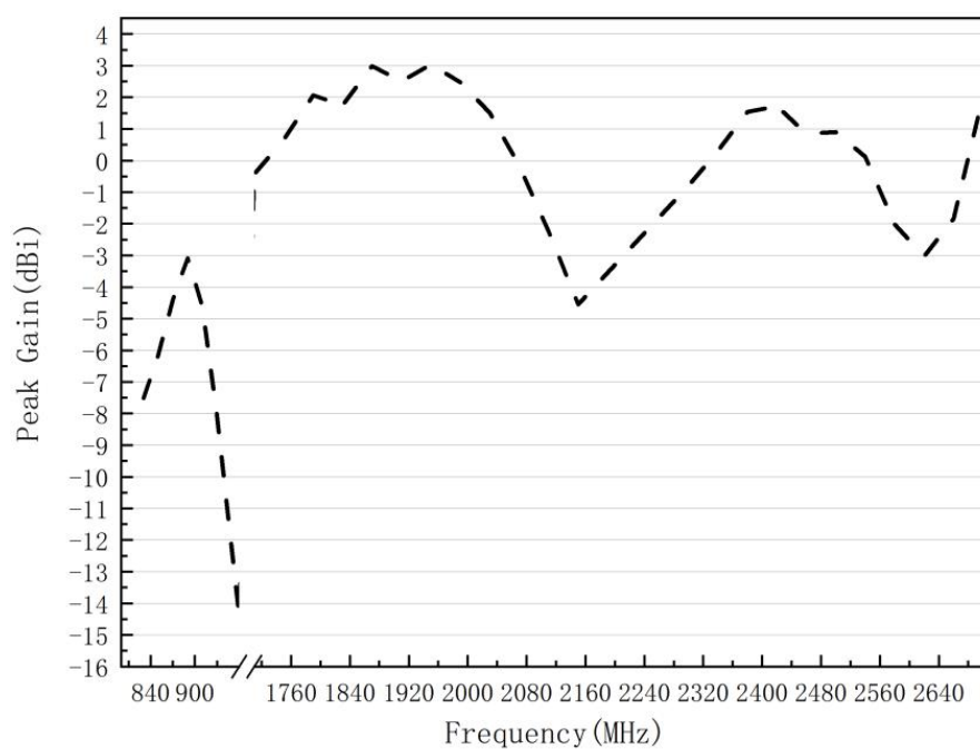
Figure 9. Peak Gain
