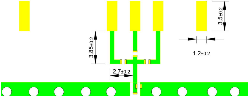
Figure 5. Matching Circuit
