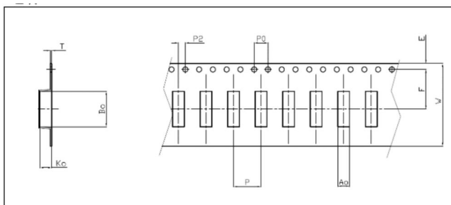
Figure 10. Packaging Information
