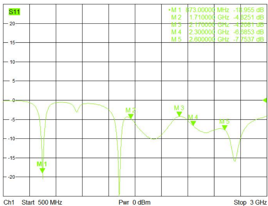
Figure 6. Return Loss
