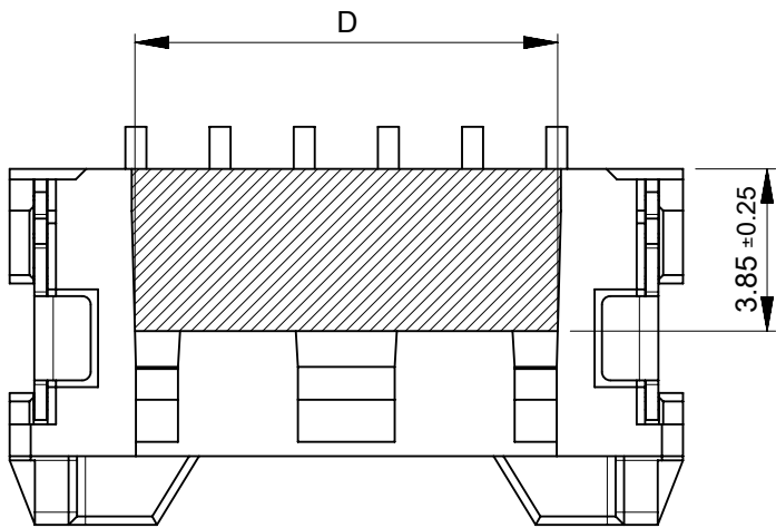
6-16 CIRCUIT
