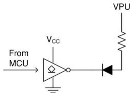
Figure 5.1: Application Schematic
