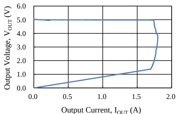
Figure 9-8. Overcurrent Protection Characteristic Example ( V_{IN} = 12 \text{ V} )
