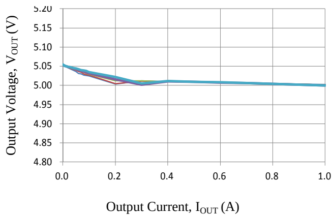
Figure 12-4. Load Regulation
