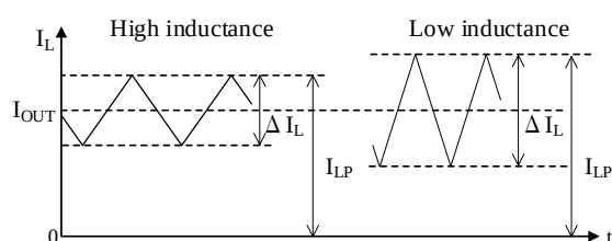
Figure 10-2 Relationship between Inductance and Ripple Current
