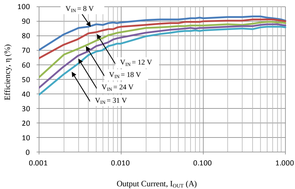
Figure 12-1. Efficiency Curves
