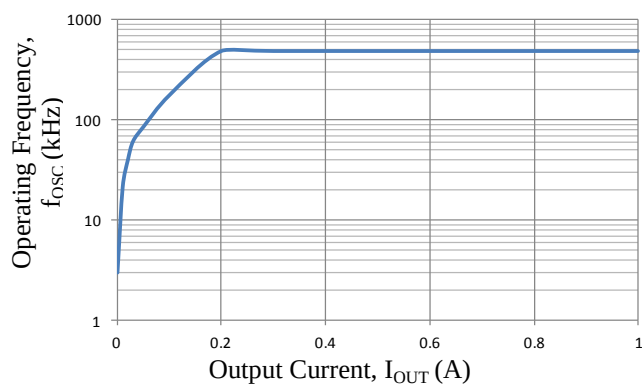
Figure 12-6. Operating Frequency
