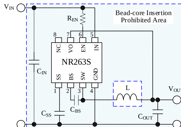
Figure 10-9. Bead-core Insertion Prohibited Area
