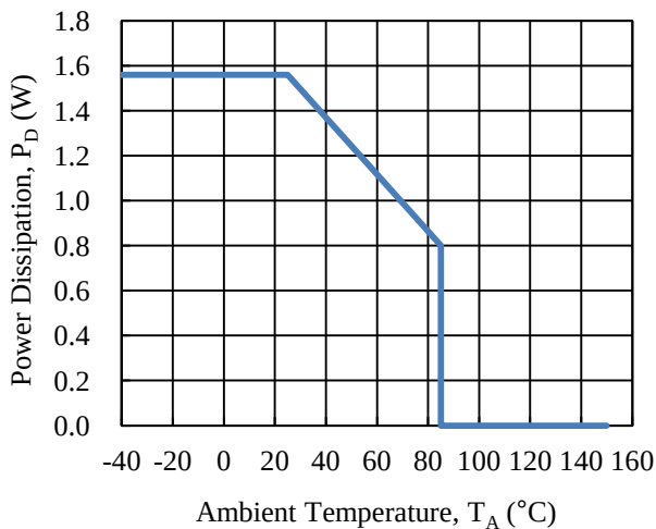
Figure 10-1. Thermal Derating Curve
