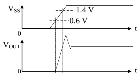
Figure 9-6. Soft-start Operational Waveform (Soft-start Period is Too Short)
