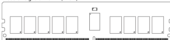
Figure 1: 288-Pin RDIMM (MO-309, R/C-C1, R/C-C2)
