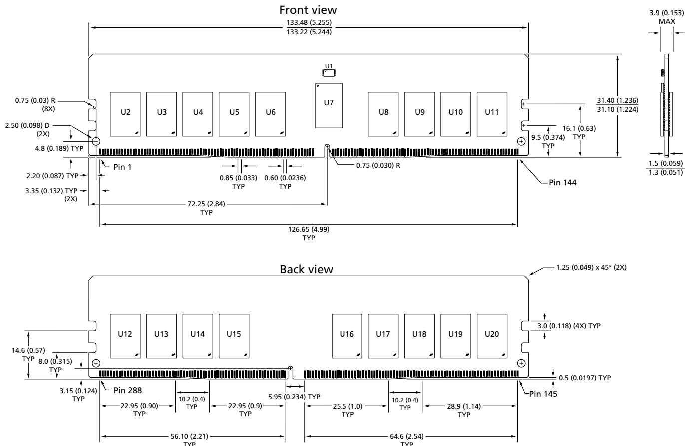
Figure 3: 288-Pin DDR4 RDIMM, R/C-C1 and C2
