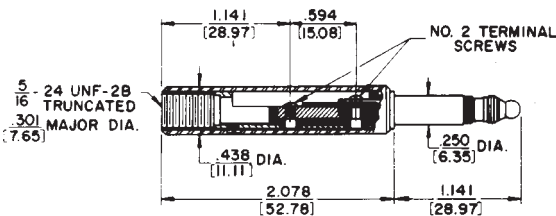
480 Series
