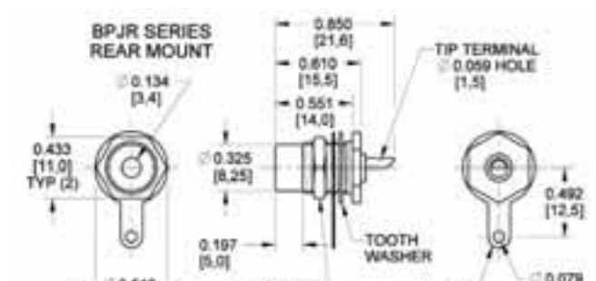
BPJR Series
