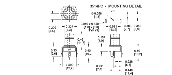
3514PC, 3517PC
