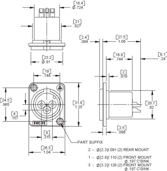
PD3MSC1AU
