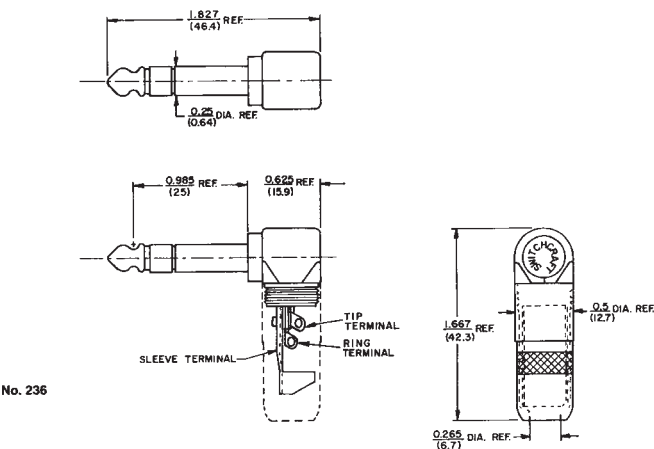
236 Right Angle 1/4" Plugs
