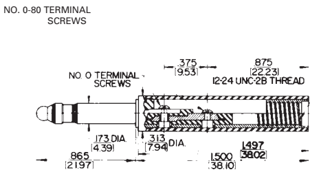
TT253 Series
