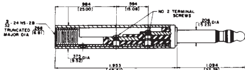
484 Series
