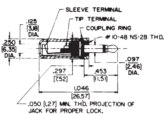
851 (typical) Series
