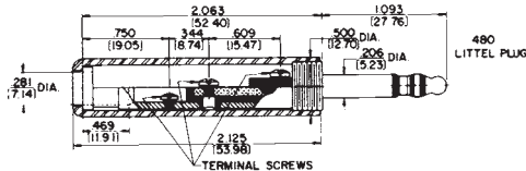
482 Series
