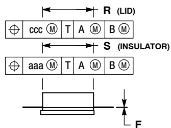
CASE 465C-02 ISSUE D NI-880S MRFE6S9135HSR3
