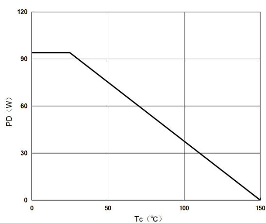
Figure 12: Power De-rating
