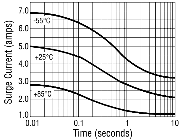
Figure 8 - Maximum Surge Current Without Tripping
