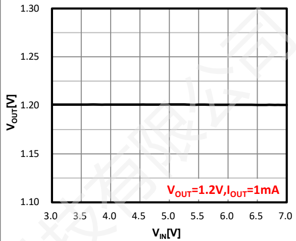
Figure 14. Line Regulation
