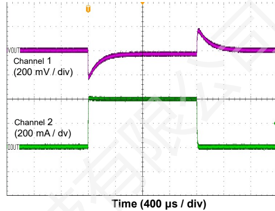
Figure 32. Load Transient (1 mA → 400 mA)
