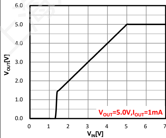
Figure 17. V_{OUT} vs V_{IN}
