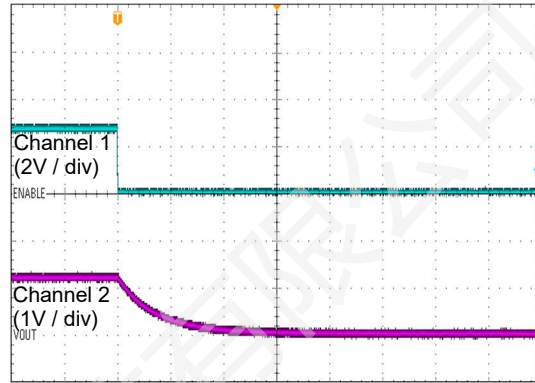
Figure 26. Shut-Down with Enable
