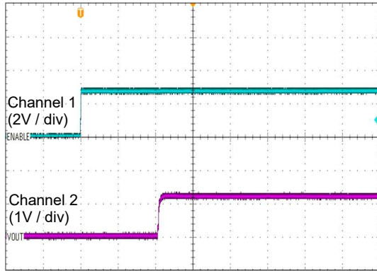
Figure 25. Power-Up with Enable
