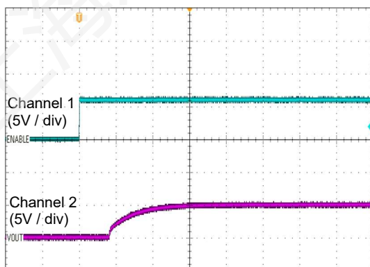
Figure 27. Power-Up with Enable
