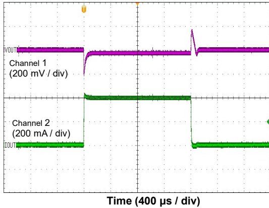
Figure 31. Load Transient (1 mA → 400 mA)
