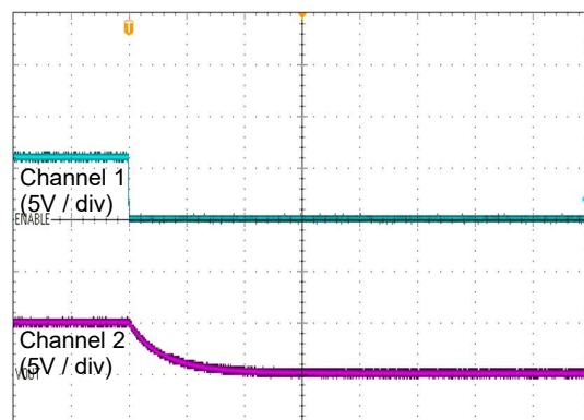
Figure 28. Shut-Down with Enable
