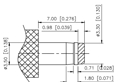
ø3.5mm DC PLUG DETAIL DRWING
