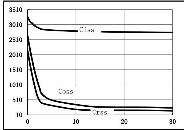
Fig.2 Capacitance Characteristics
