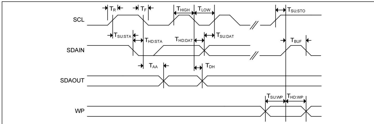
Figure 1-11. Bus Timing
