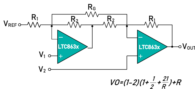
Figure 9: Instrumentation Amplifier
