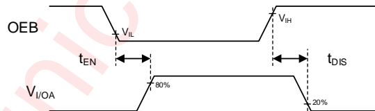
t_{EN} and t_{DIS} Timing For OEB
