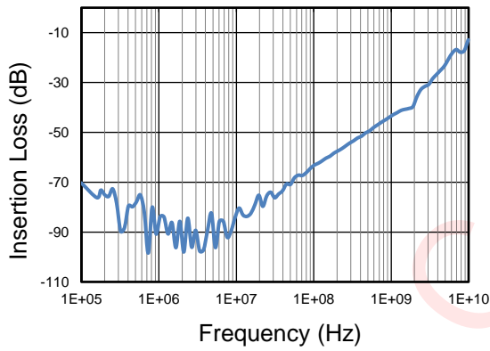
Differential Crosstalk
