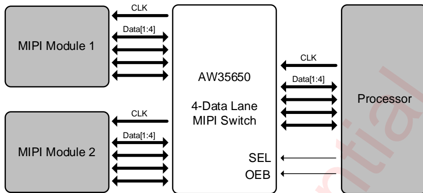
Typical Application Circuit of AW35650
