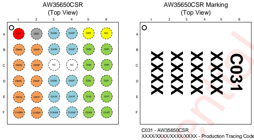
Pin Configuration and Top Mark
