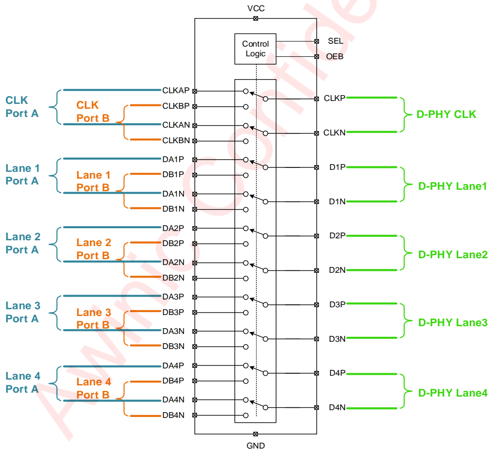
Recommended D-PHY Configuration of AW35650
