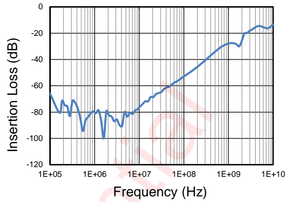
Off Isolation
