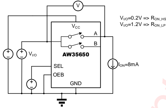
On Resistance
