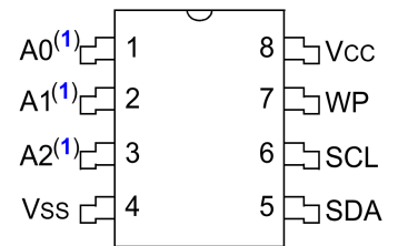
SOIC, TSSOP (Top View)
