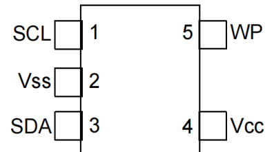
SOT-23 (Top View)
