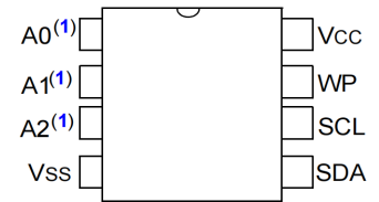
PDIP (Top View)
