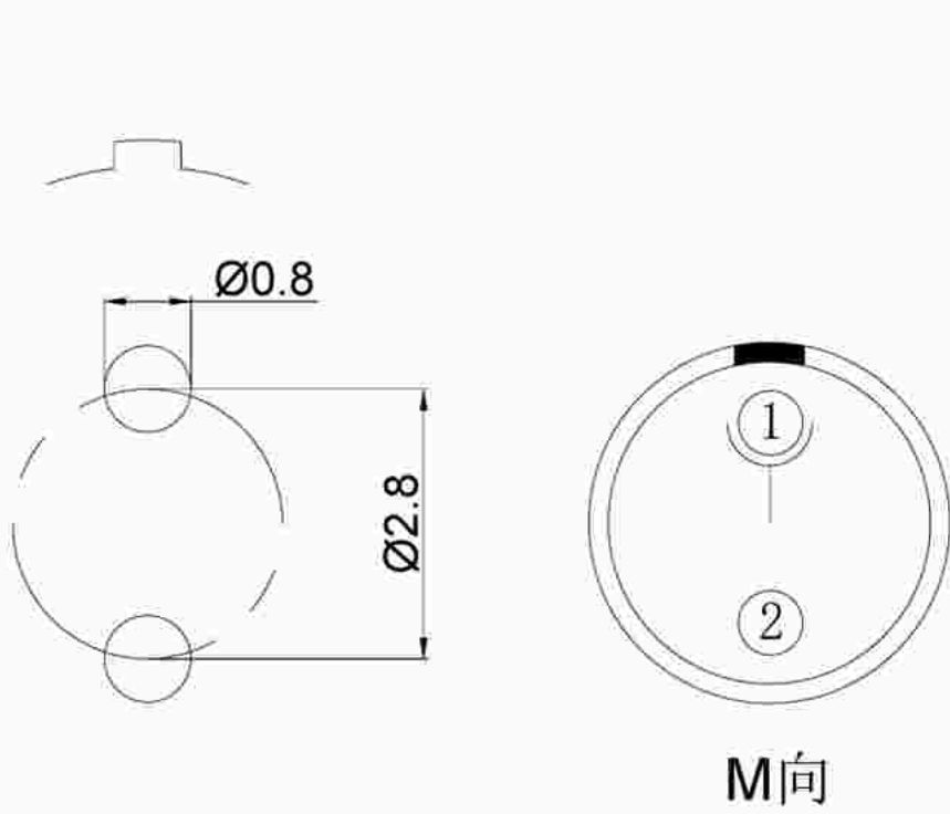
Pcb plate opening size (PCB板开孔尺寸)
