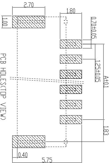
GENERAL TOLERANCE:±0.05mm
