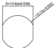
Pane hole size (面板开孔尺寸)
