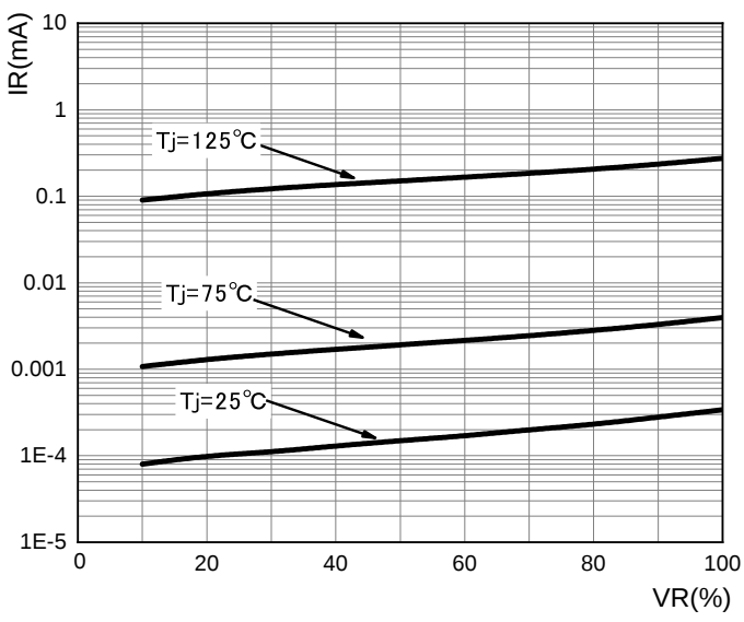
FIG.8: TYPICAL REVERSE CHARACTERISTICS
