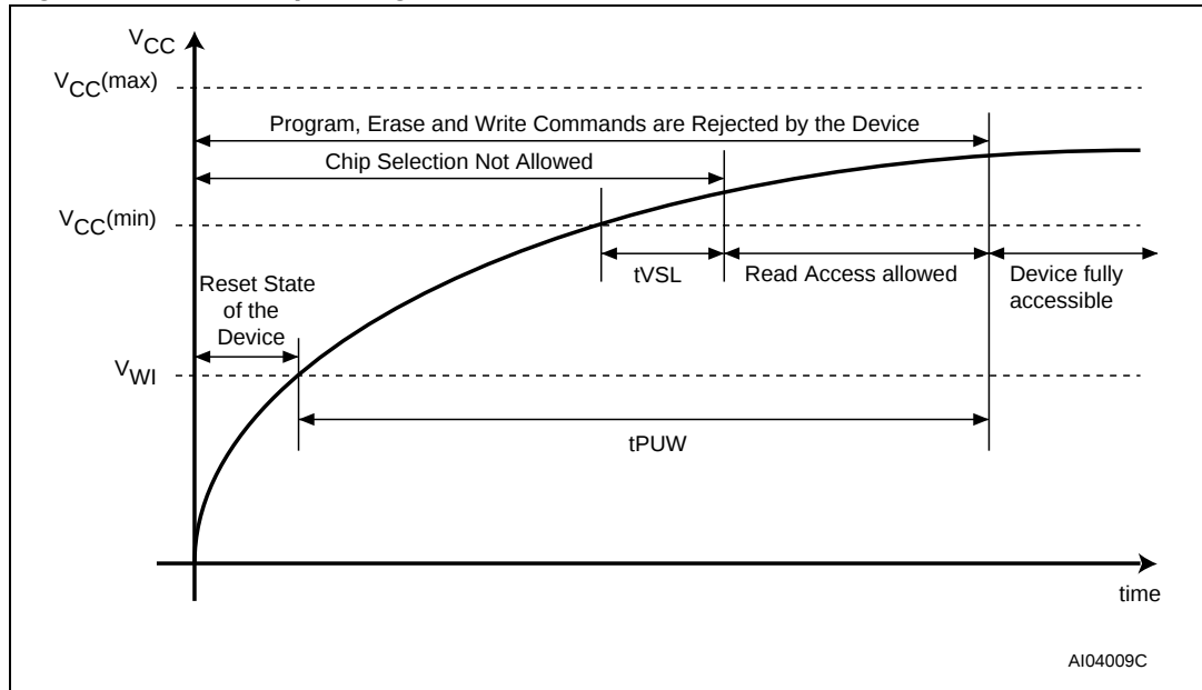
Figure 18. Power-up timing
