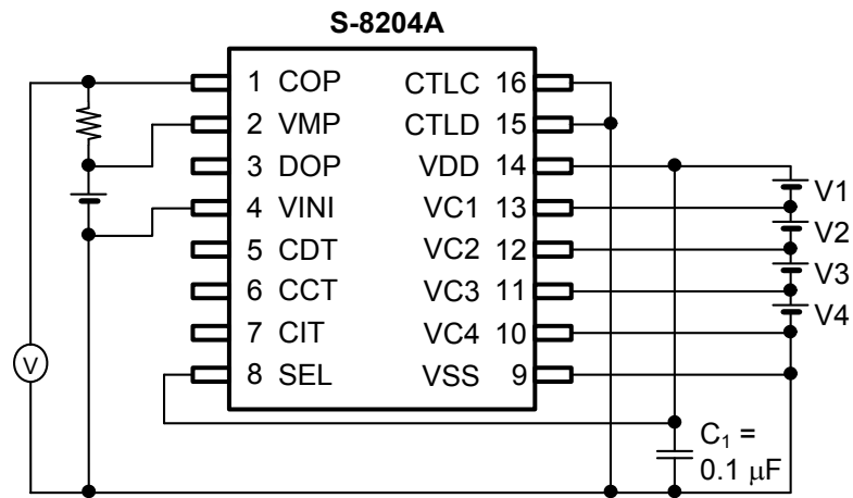
Figure 7 Test Circuit 4
