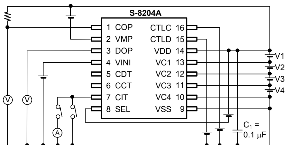
Figure 5 Test Circuit 2
