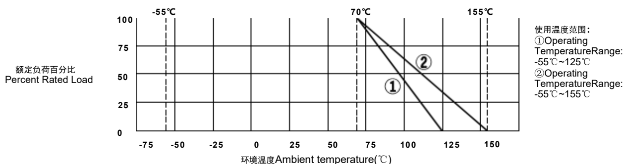
*负荷下降曲线Derating Curve
