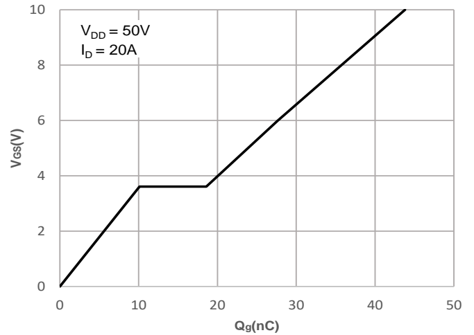
Fig.4 Gate-Charge Characteristics
