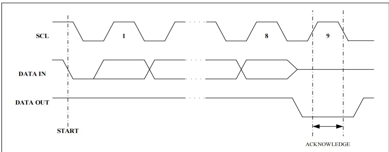
Figure 4. Output Acknowledge
