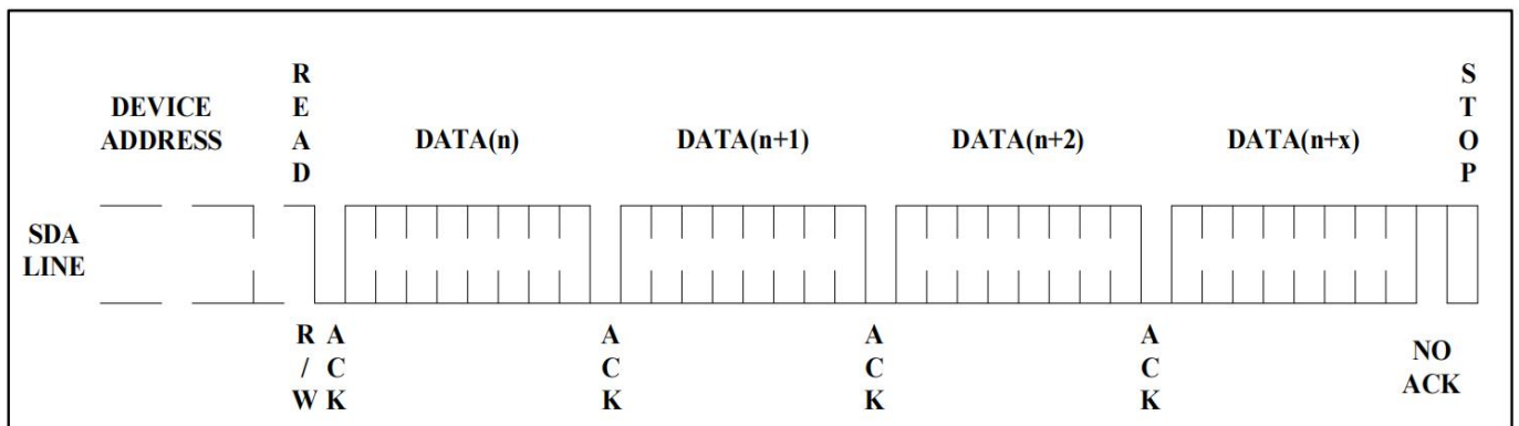
Figure 10. Sequential Read
