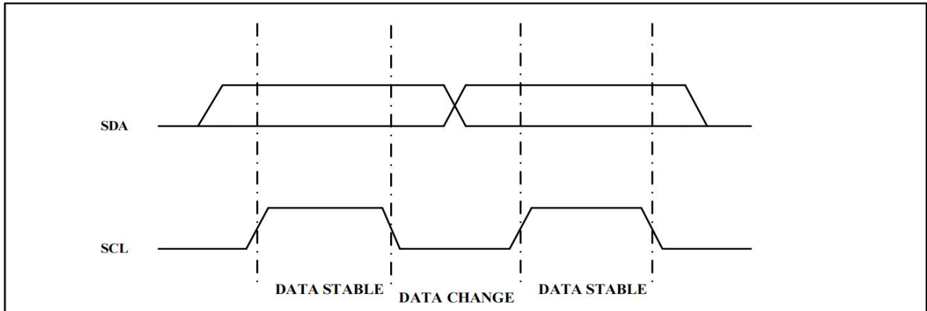
Figure 2. Data Validity
