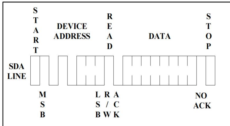
Figure 9. Random Read
