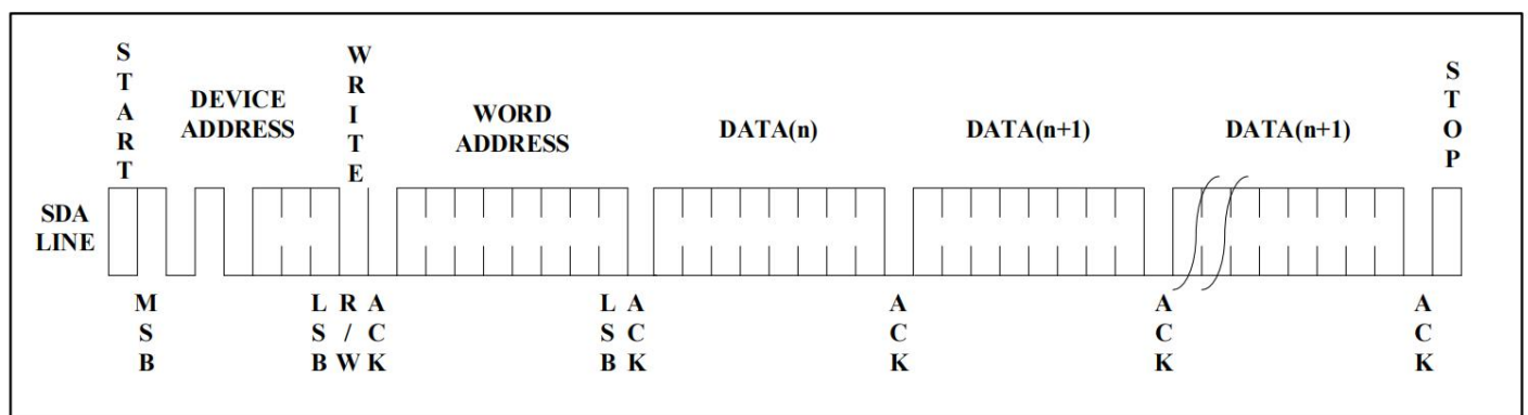
Figure 7. Page Write
