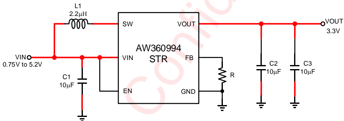
Typical Application Circuit of AW360994STR
