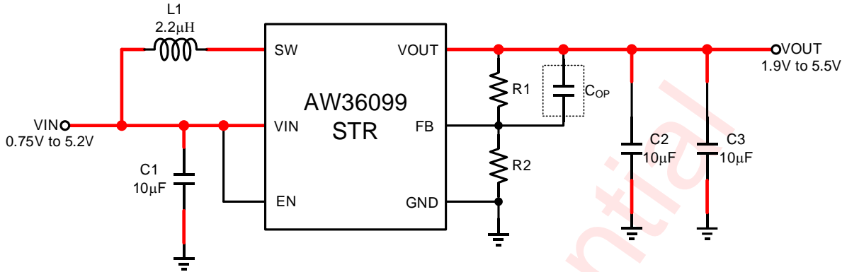
Typical Application Circuit of AW36099STR
