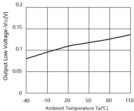
Fig.5 Output Low Voltage vs Ambient Temperature
