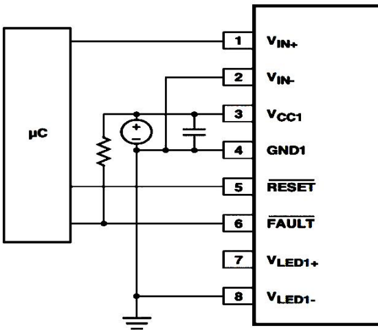
Figure 64. Local shutdown, local reset configuration
