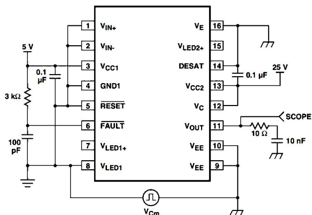
Fig47. CMR test circuit,LED1 off
