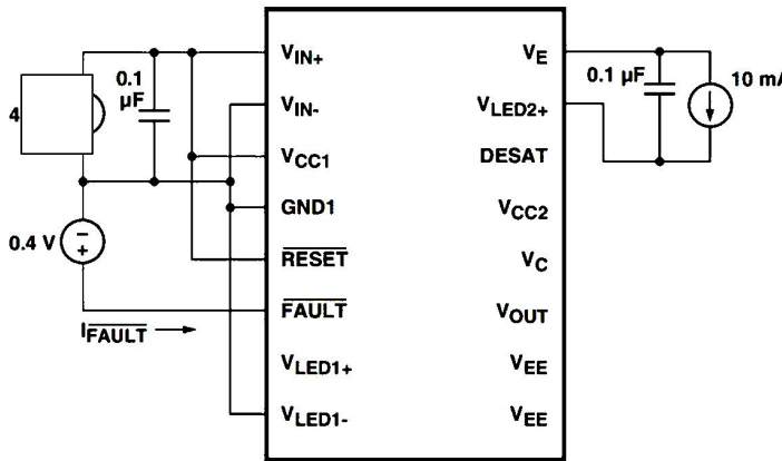
Fig25. IFAULTL test circuit
