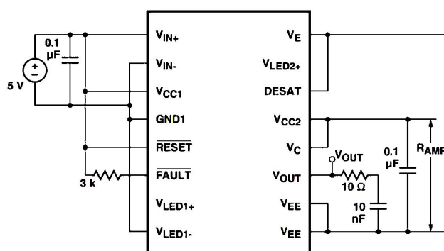
Fig44. UVLO delay test circuit
