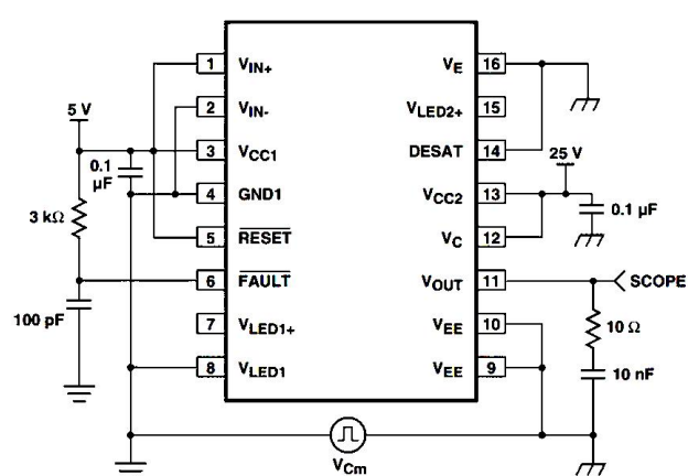
Fig48. CMR test circuit,LED1 on
