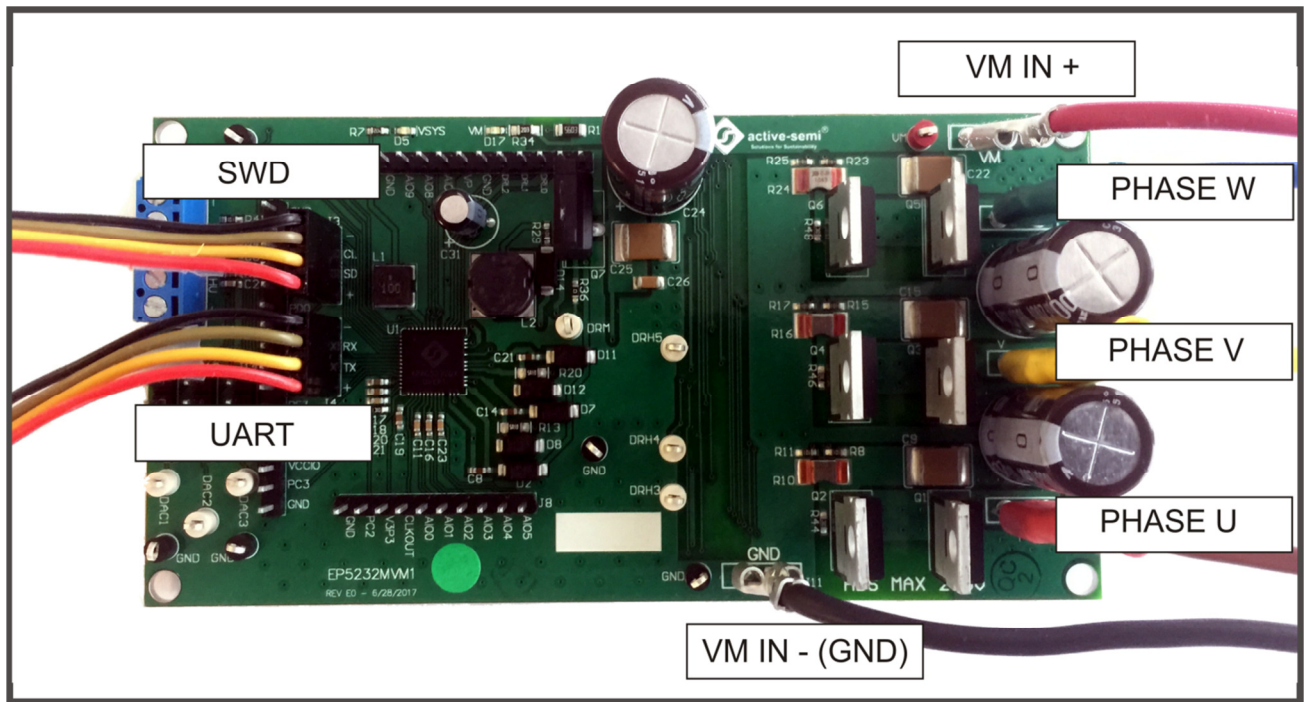
Figure 7: PAC5232EVK1 Evaluation Module Connections
