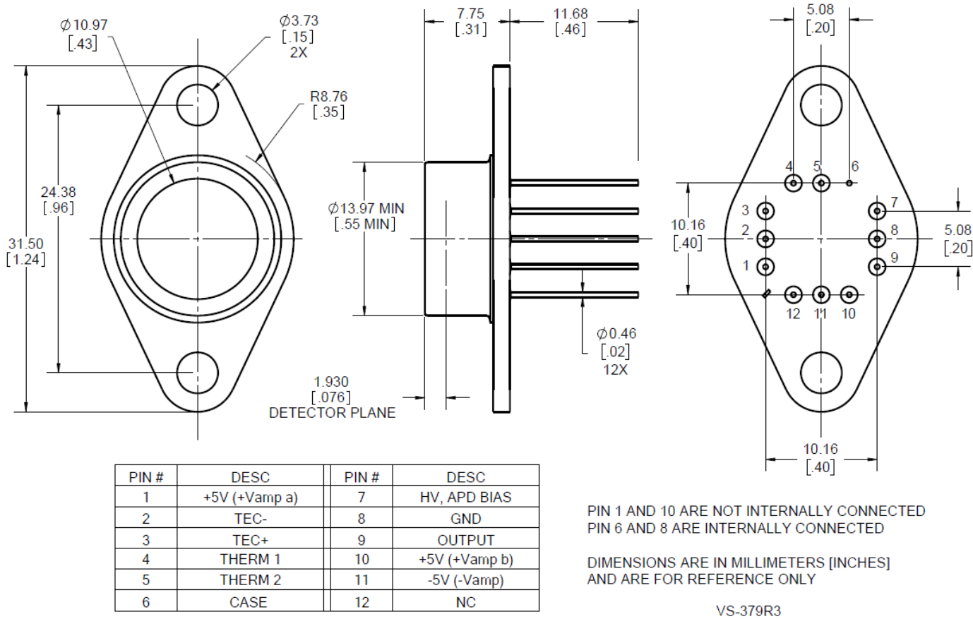
Figure 7. Mechanical Characteristics – LLAM Series – reference dimensions shown in mm [inches]
