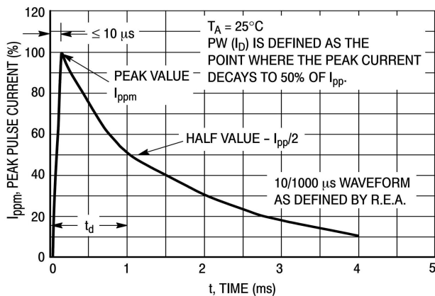
Figure 11. Pulse Waveform
