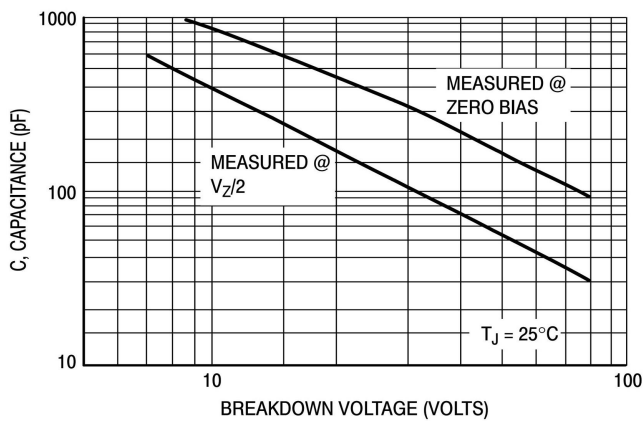
Figure 9. Capacitance Curve
