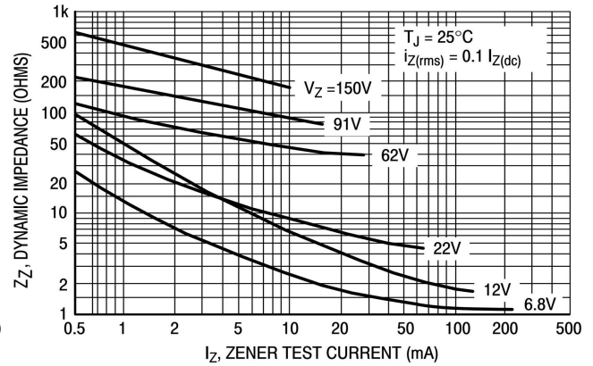
Figure 8. Effect of Zener Current
