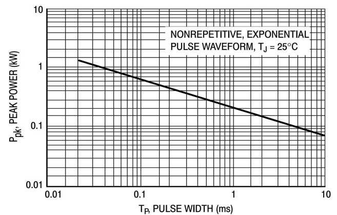
Figure 10. Typical Pulse Rating Curve
