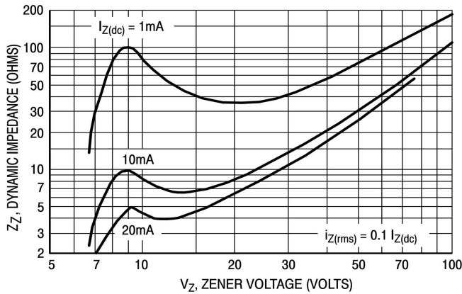
Figure 7. Effect of Zener Voltage
