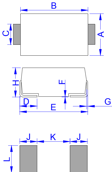
DO-214AA (SMB)
