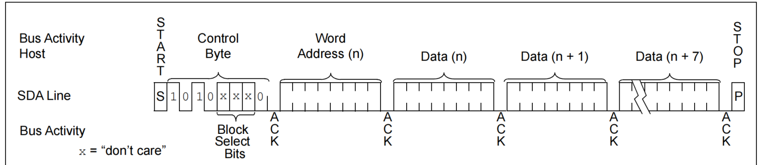
FIGURE 6-2: PAGE WRITE
