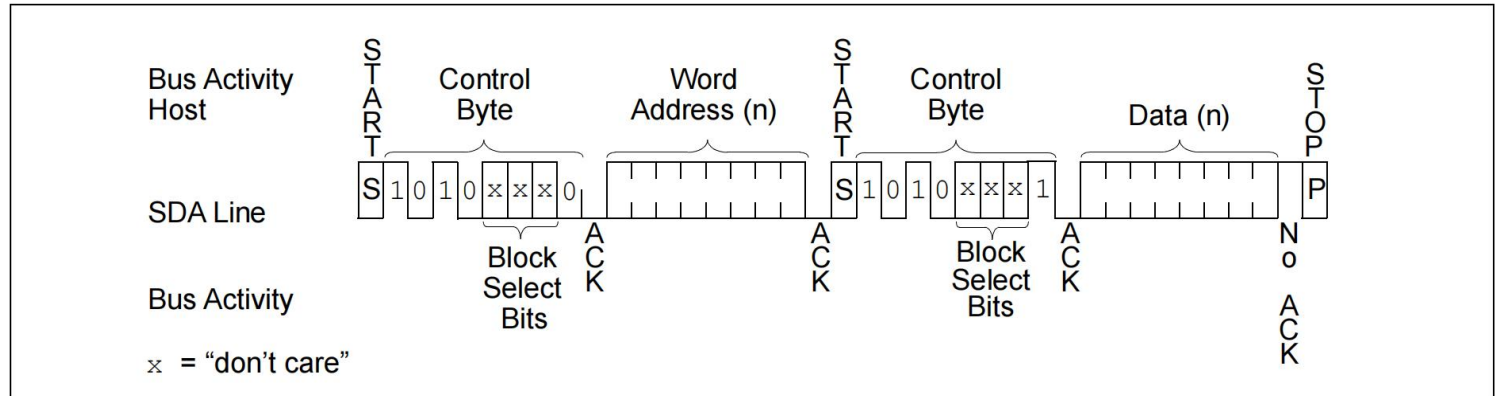
FIGURE 8-2: RANDOM READ
