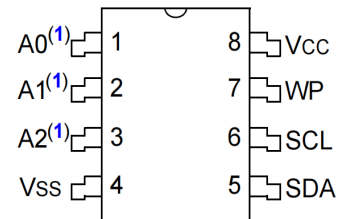
SOIC, TSSOP (Top View)
