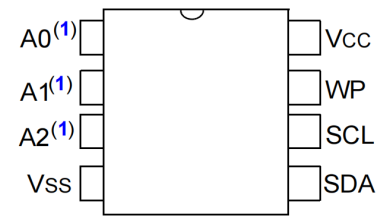
PDIP (Top View)
