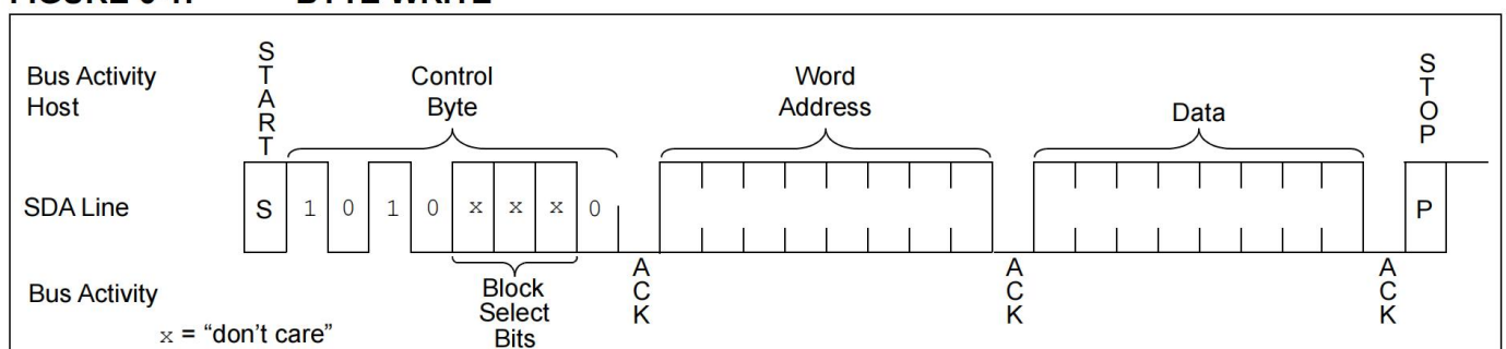
FIGURE 6-1: BYTE WRITE
