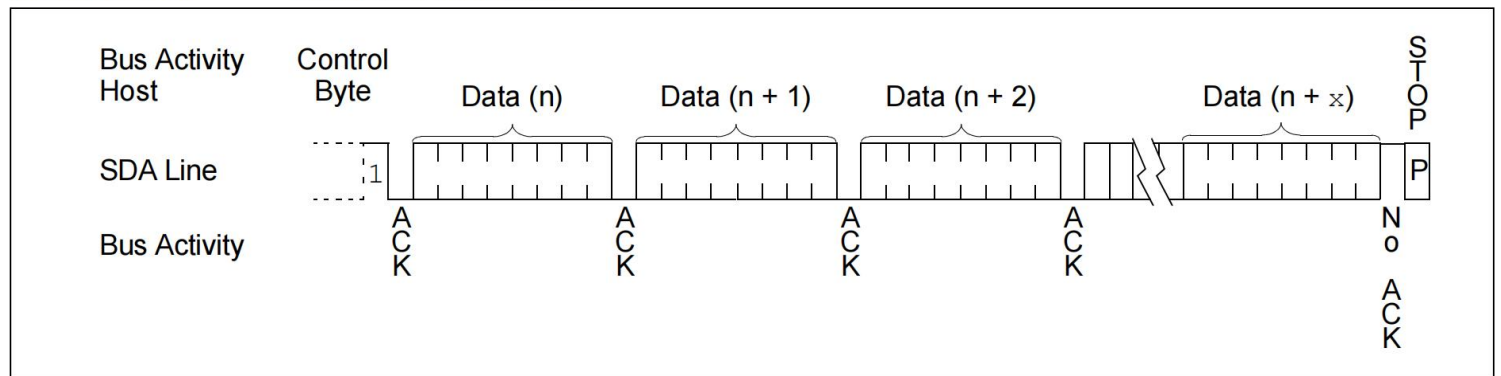
FIGURE 8-3: SEQUENTIAL READ
