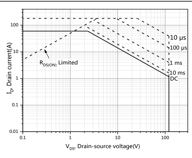
Figure 10, Safe operation area for TO220 T_C=25\text{ }^\circ\text{C}
