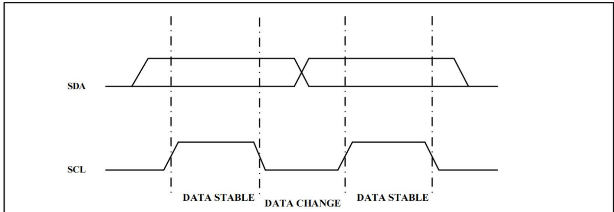
Figure 2. Data Validity
