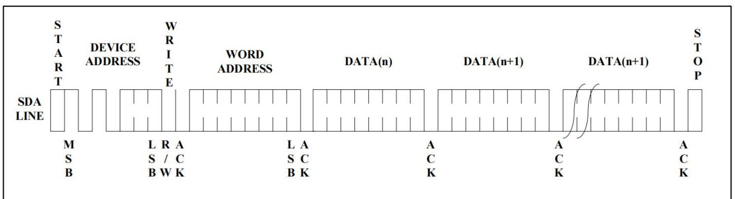
Figure 7. Page Write
