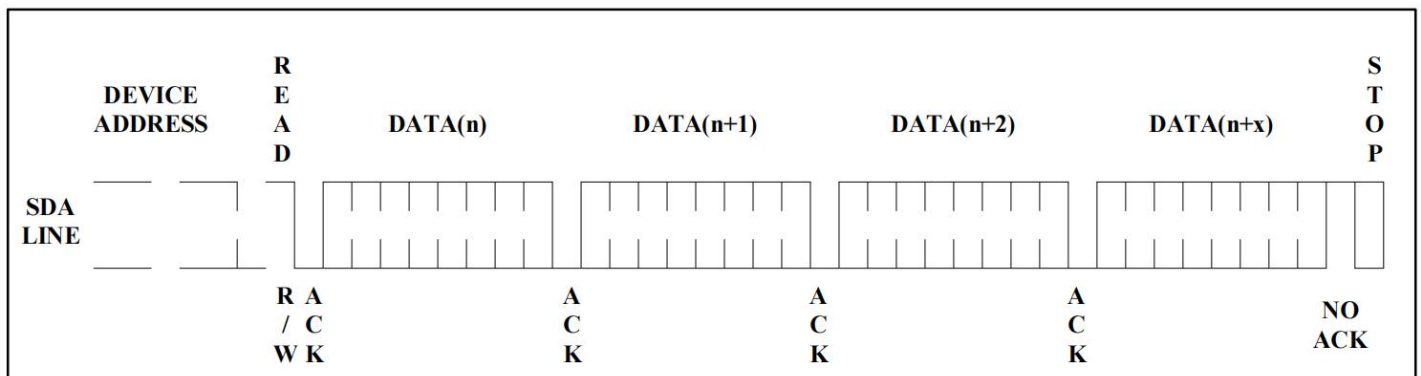
Figure 10. Sequential Read
