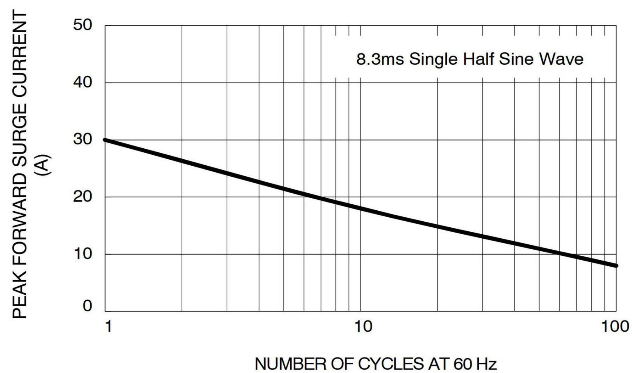
Figure 3. Maximum Non-Repetitive Forward Surge Current
