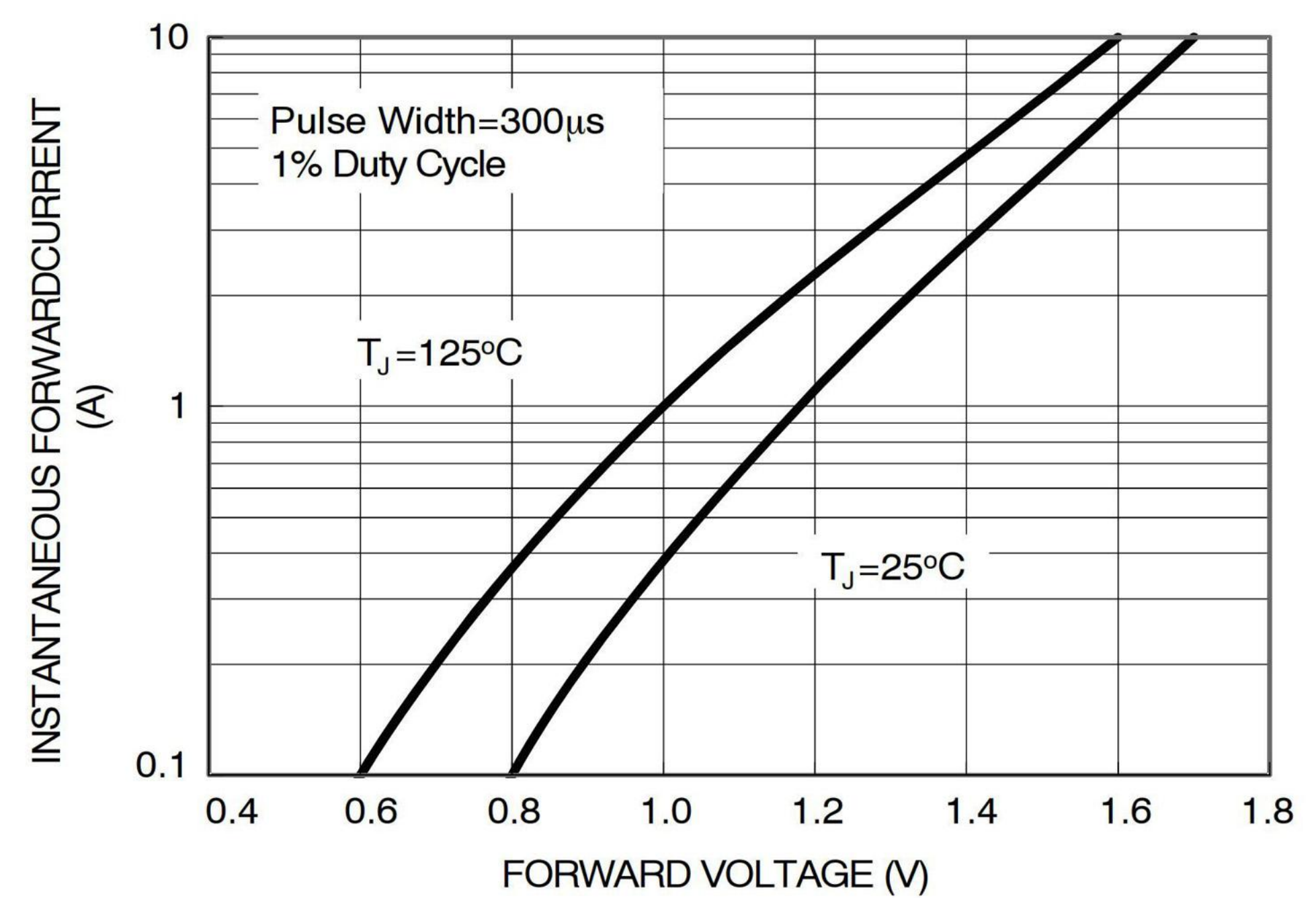
Figure 4. Typical Instantaneous Forward Characteristics
