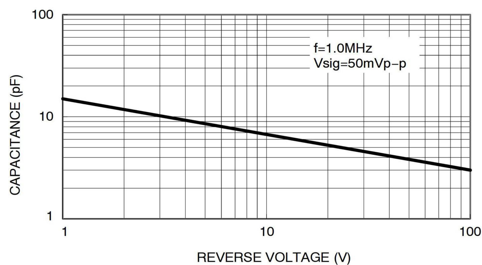
Figure 5. Typical Junction Capacitance
