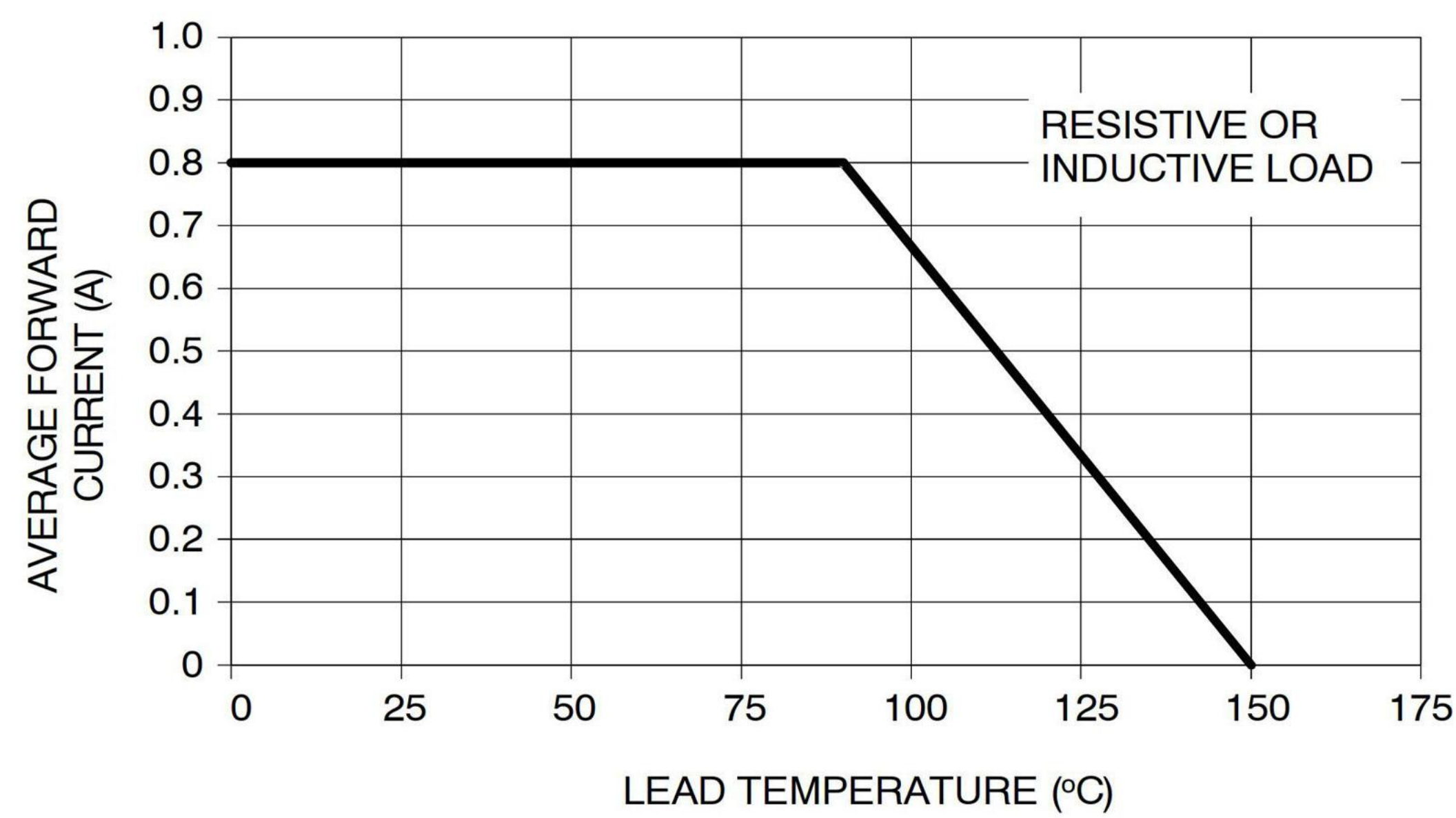
Figure 1. Forward Current Derating Curve
