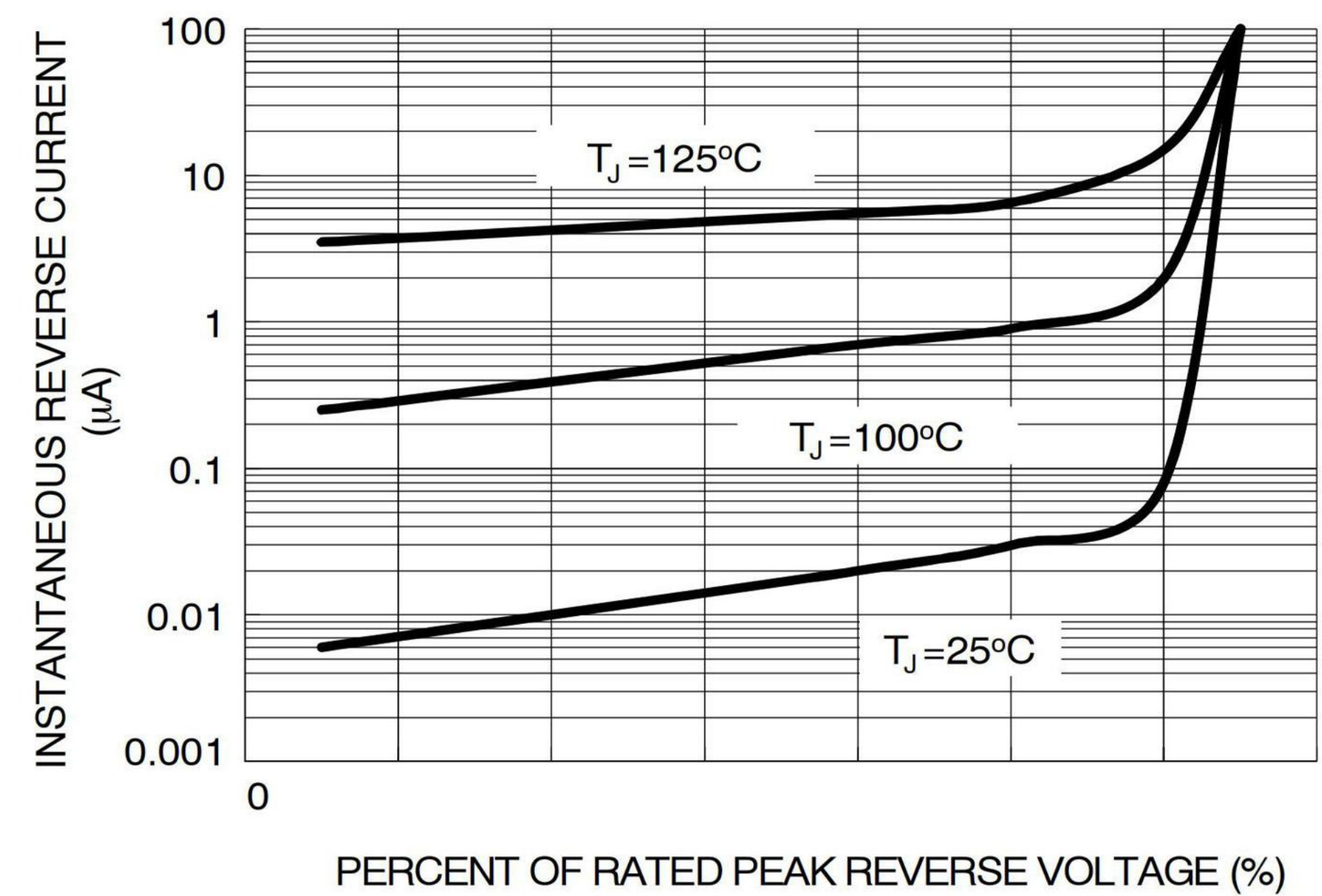
Figure 2. Typical Reverse Characteristics
